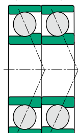
DT arrangement (tandem)
